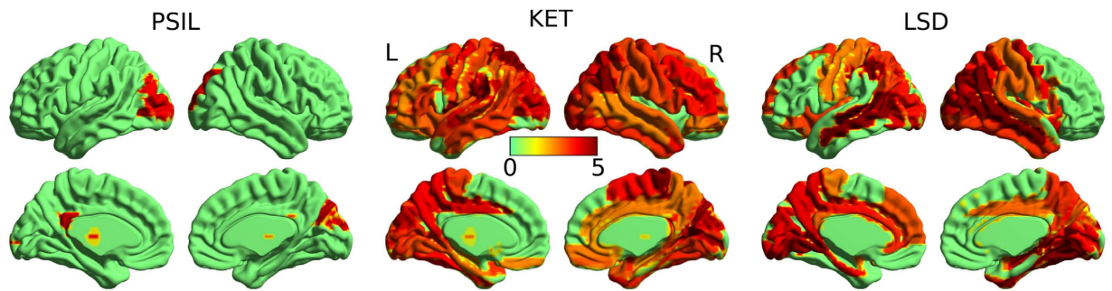
Figure 3. t -statistics across participants of \Delta LZs_N per source channel. Group level changes in single channel Lempel-Ziv complexity, \Delta LZs_N , are indicated by the t -statistic for each of the 90 source channels and 3 drugs (where significant at the p < 0.05 level, FDR corrected). For all three drugs, an increase in LZs_N can be seen in occipital-parietal areas. Image created using BrainNet viewer 55 .
